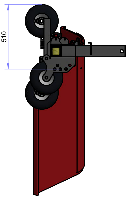
SIDE VIEW ( 1 : 15 )
