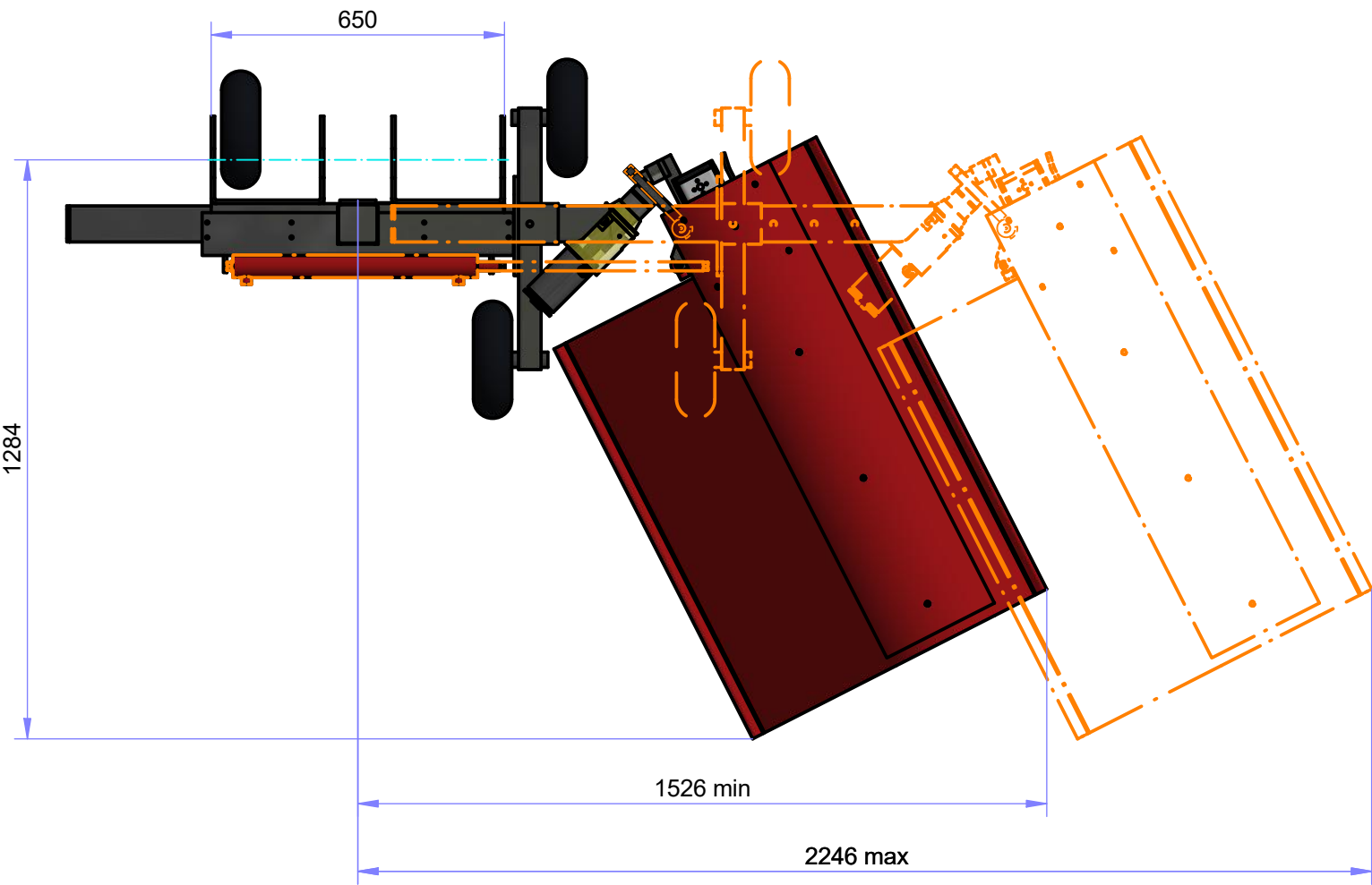
TOP VIEW ( 1 : 15 )
