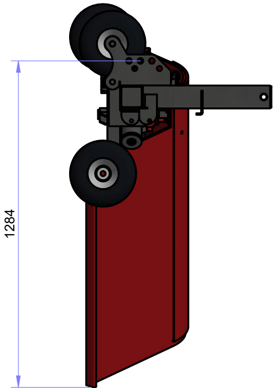
SIDE VIEW ( 1 : 15 )
