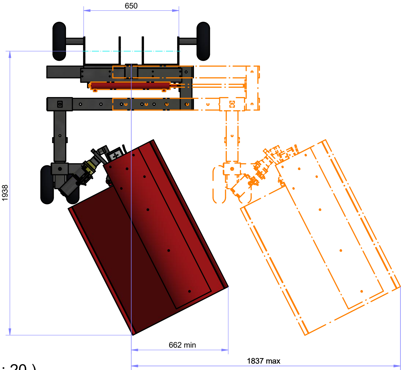
TOP VIEW ( 1 : 15 )
