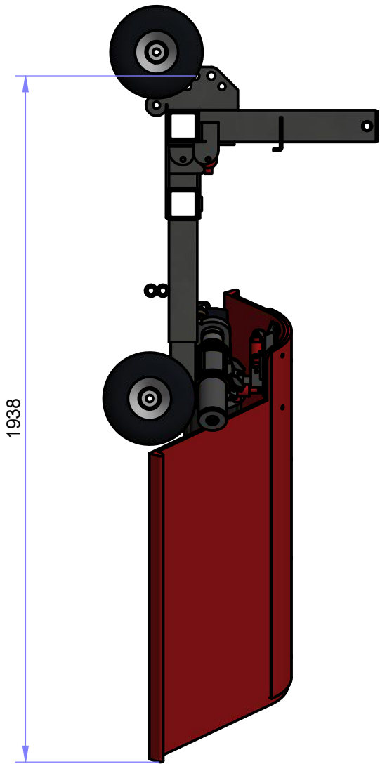
SIDE VIEW ( 1 : 15 )
