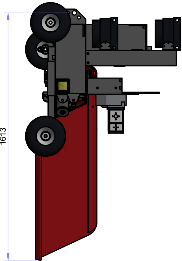
SIDE VIEW ( 1 : 15 )
