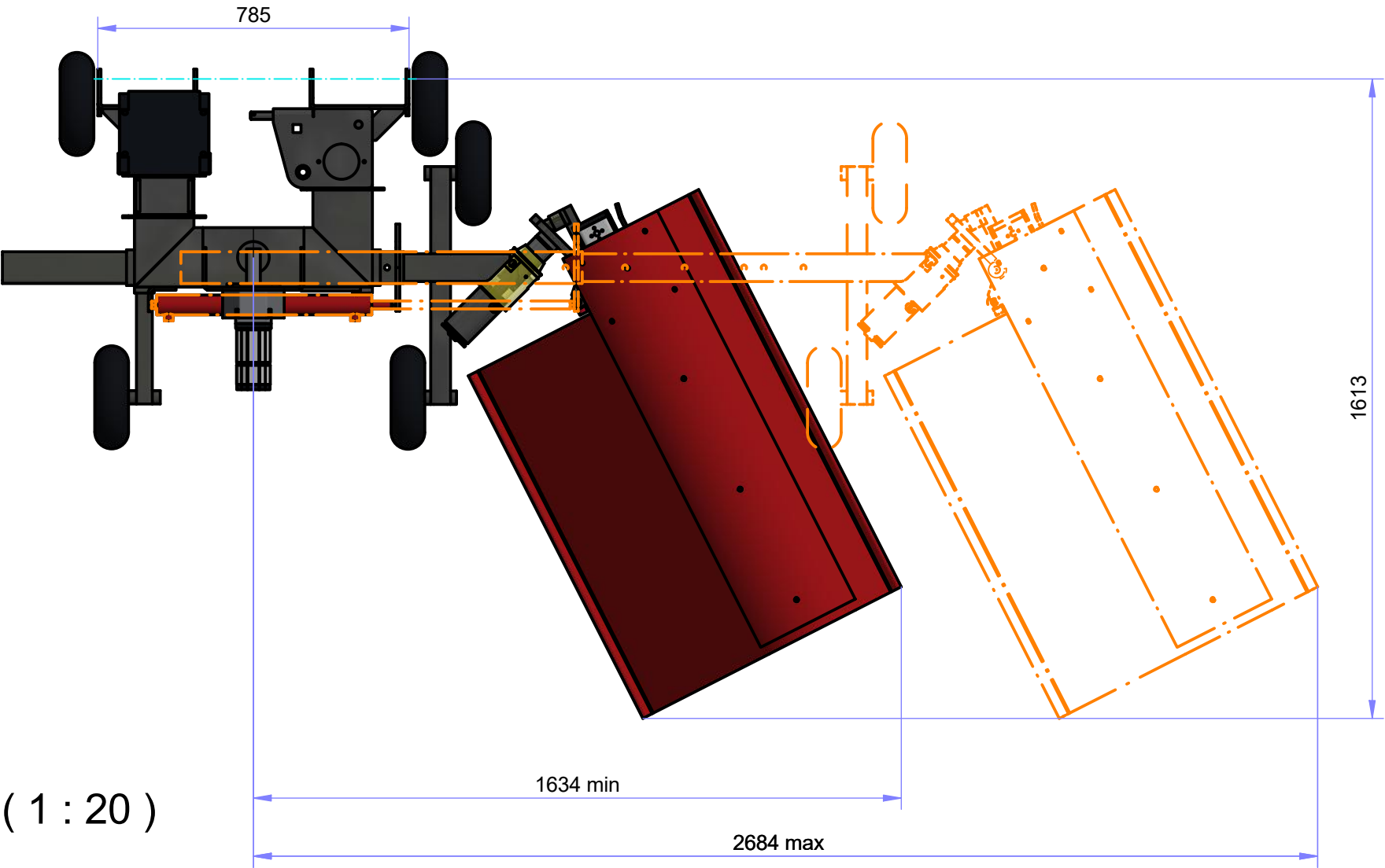
TOP VIEW ( 1 : 15 )
