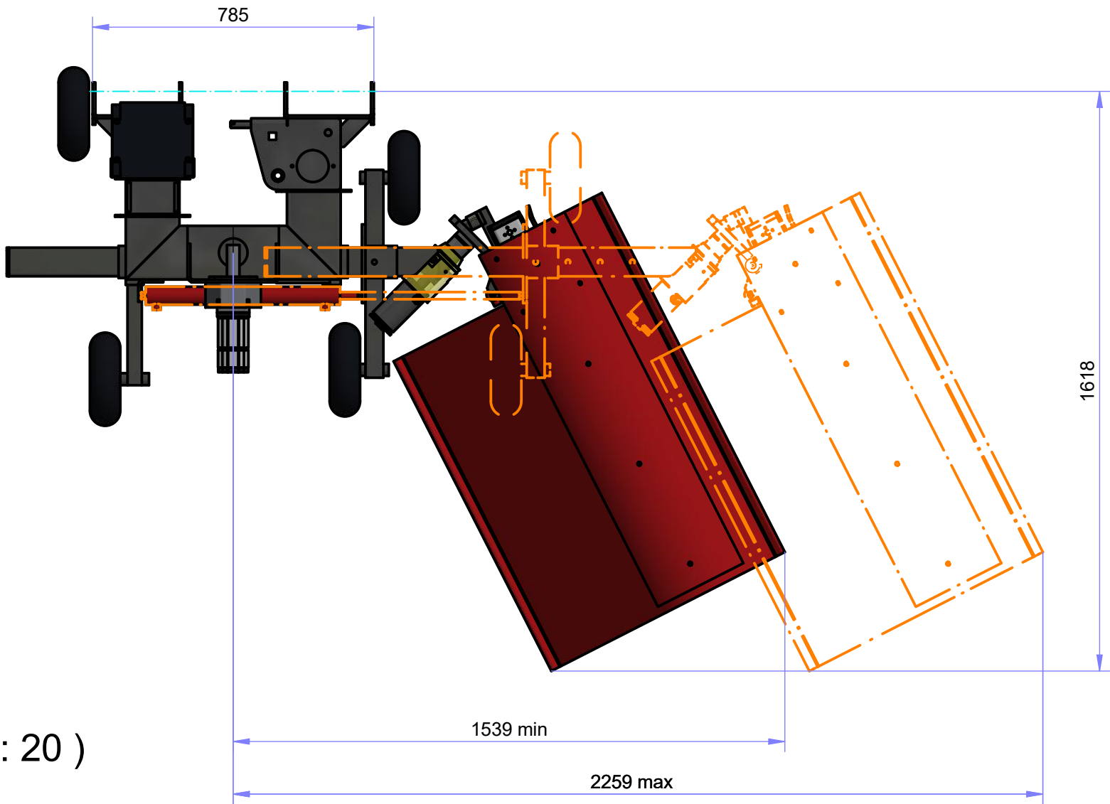
TOP VIEW ( 1 : 15 )
