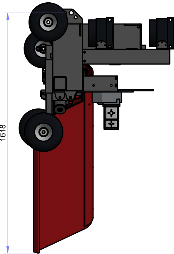
SIDE VIEW ( 1 : 15 )
