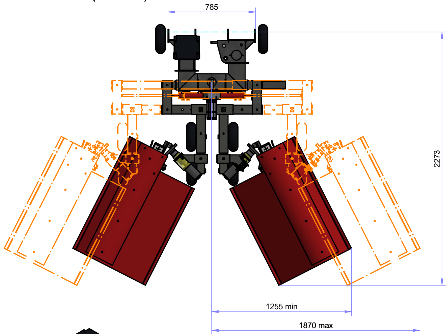
TOP VIEW ( 1 : 20 )
