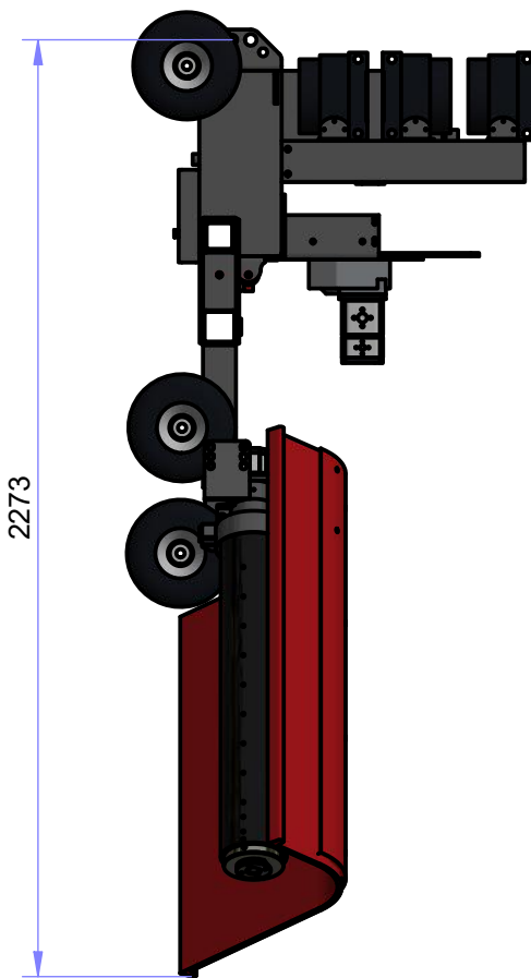
SIDE VIEW ( 1 : 20 )
