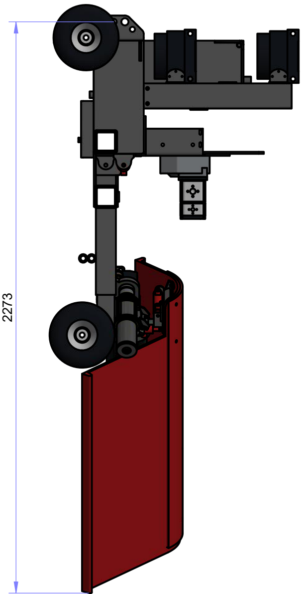
SIDE VIEW ( 1 : 15 )
