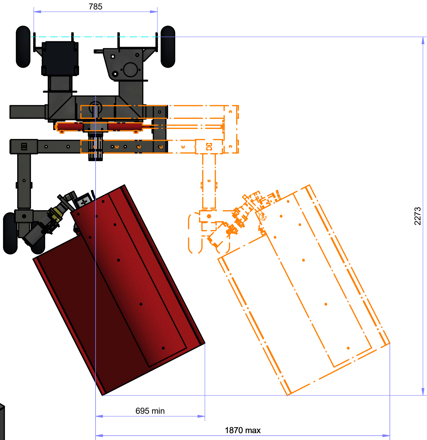
TOP VIEW ( 1 : 15 )
