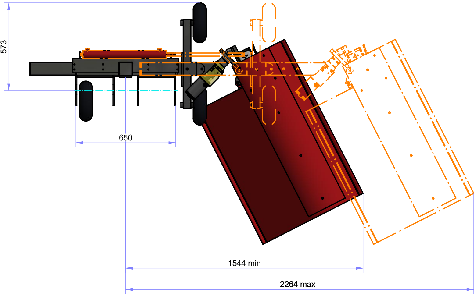
TOP VIEW ( 1 : 15 )
