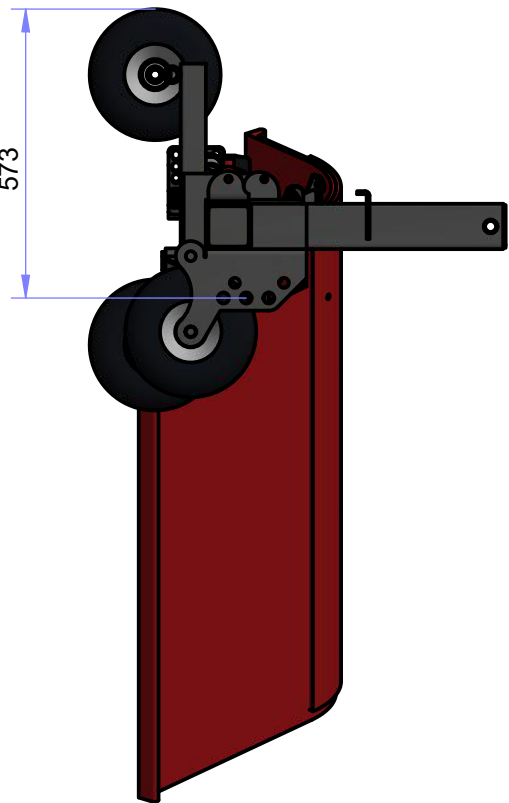
SIDE VIEW ( 1 : 15 )
