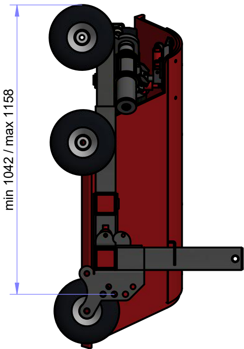
SIDE VIEW ( 1 : 15 )
