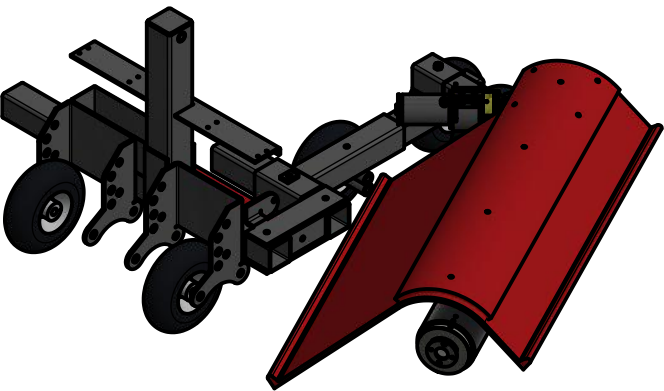
ISO VIEW ( 1 : 20 )
