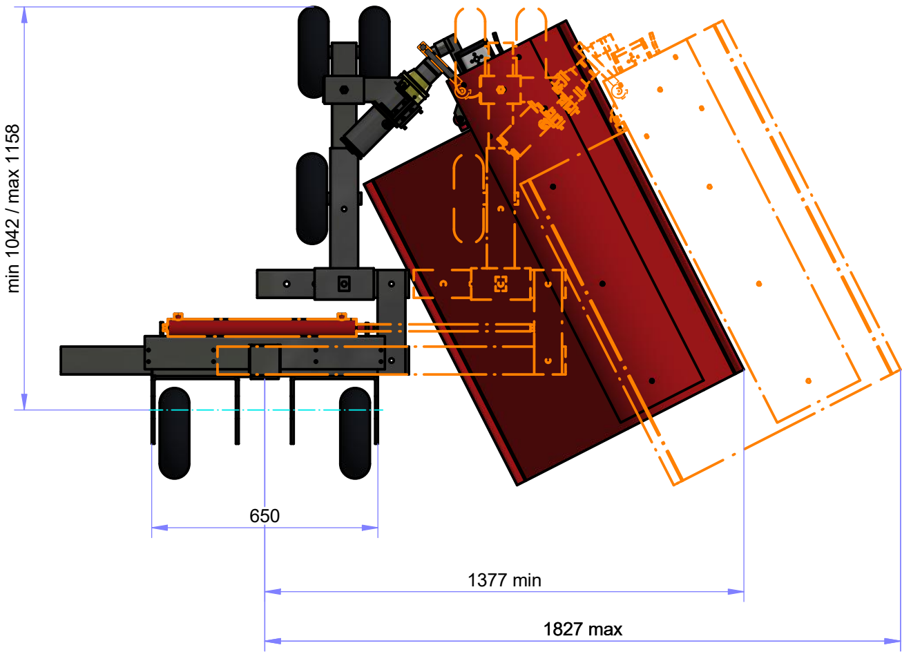
TOP VIEW ( 1 : 15 )
