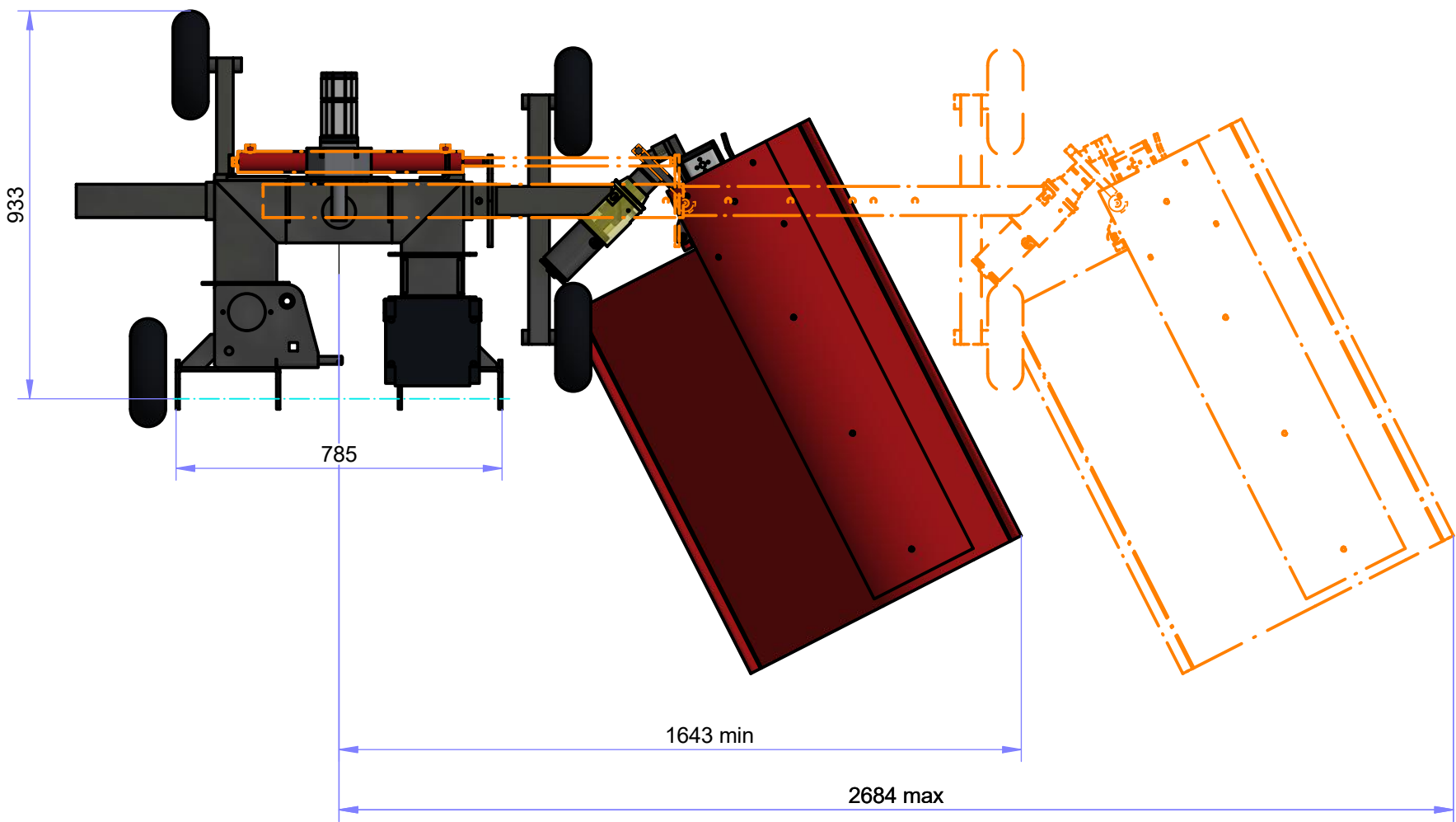
TOP VIEW ( 1 : 15 )
