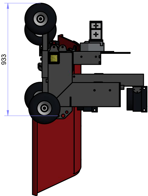
SIDE VIEW ( 1 : 15 )
