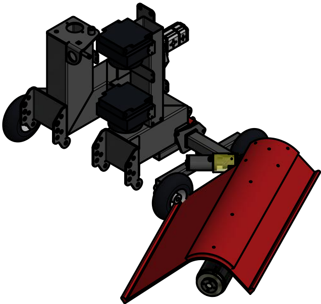
ISO VIEW ( 1 : 20 )
