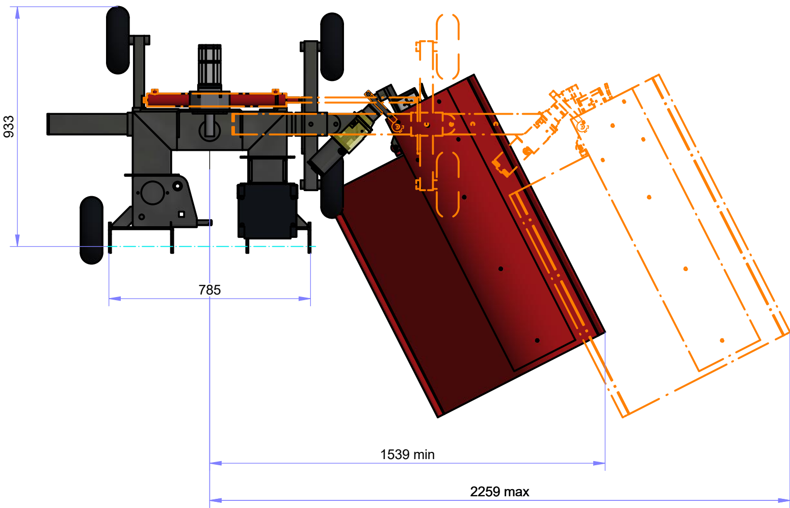
TOP VIEW ( 1 : 15 )
