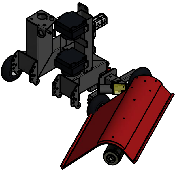
ISO VIEW ( 1 : 20 )
