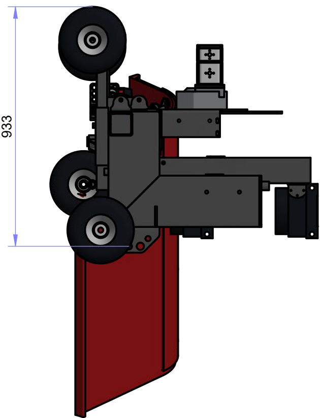
SIDE VIEW ( 1 : 15 )
