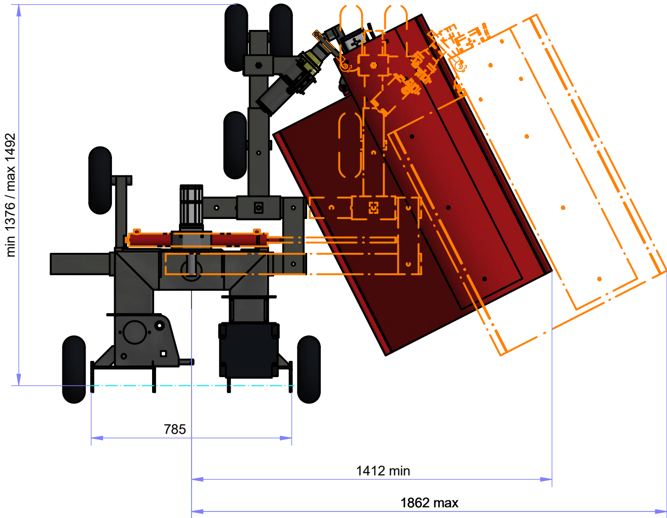
TOP VIEW ( 1 : 15 )
