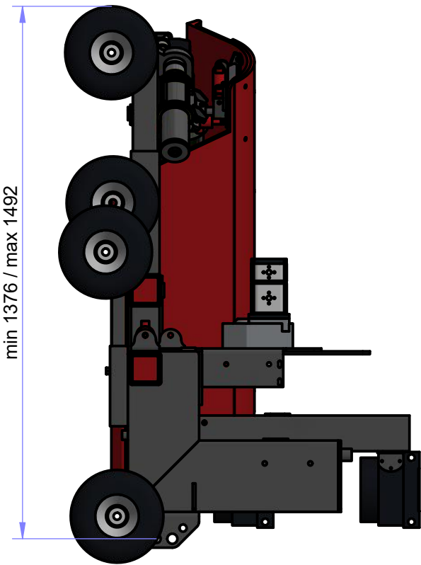
SIDE VIEW ( 1 : 15 )
