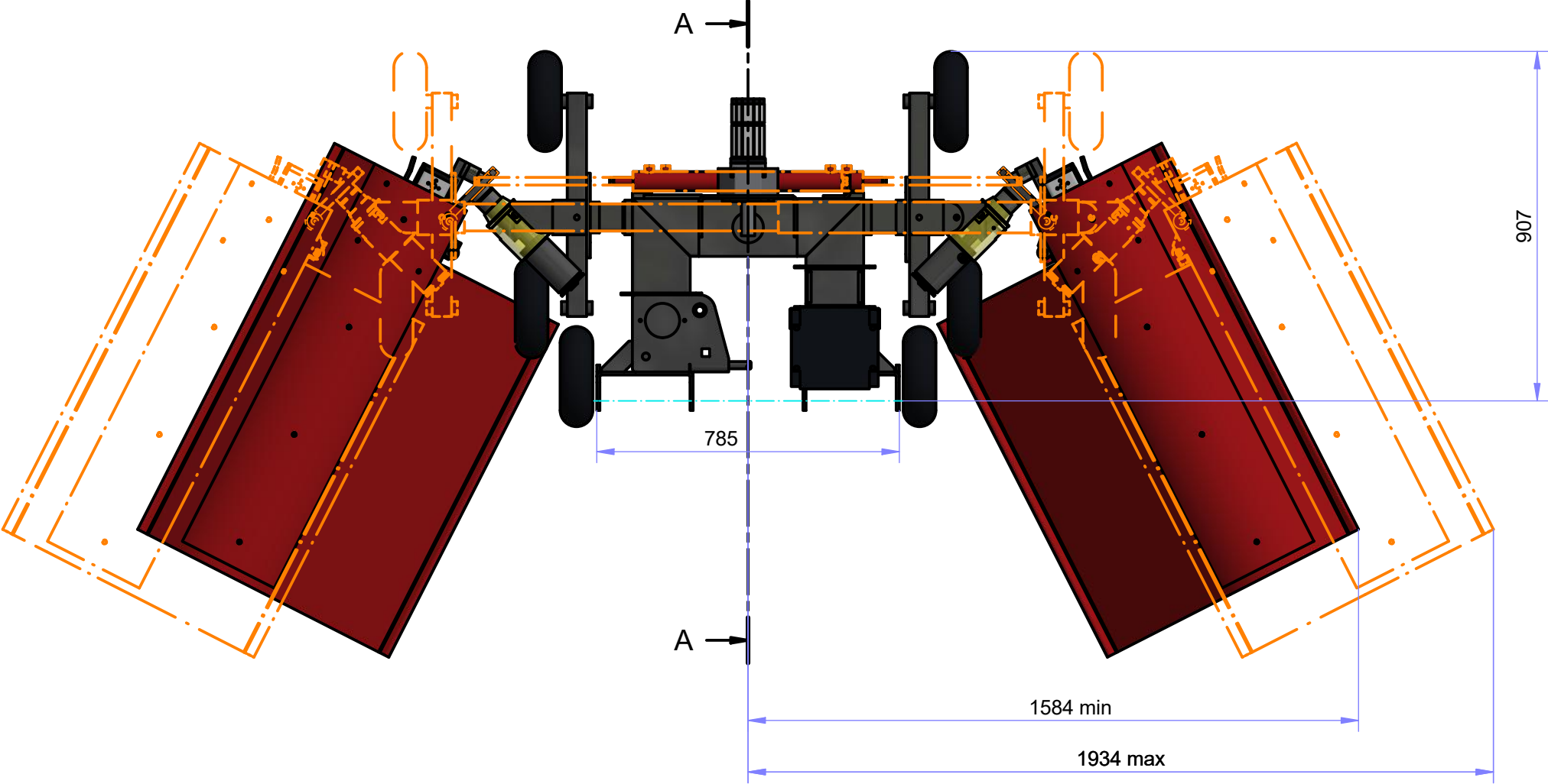
TOP VIEW ( 1 : 15 )
