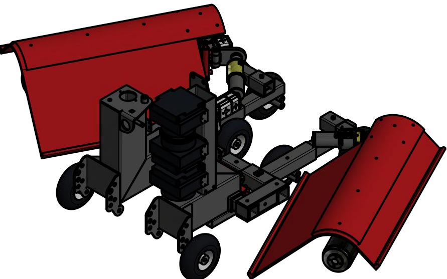
ISO VIEW ( 1 : 20 )
