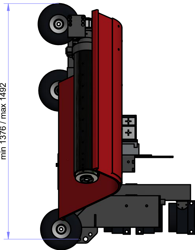
SIDE VIEW ( 1 : 15 )
