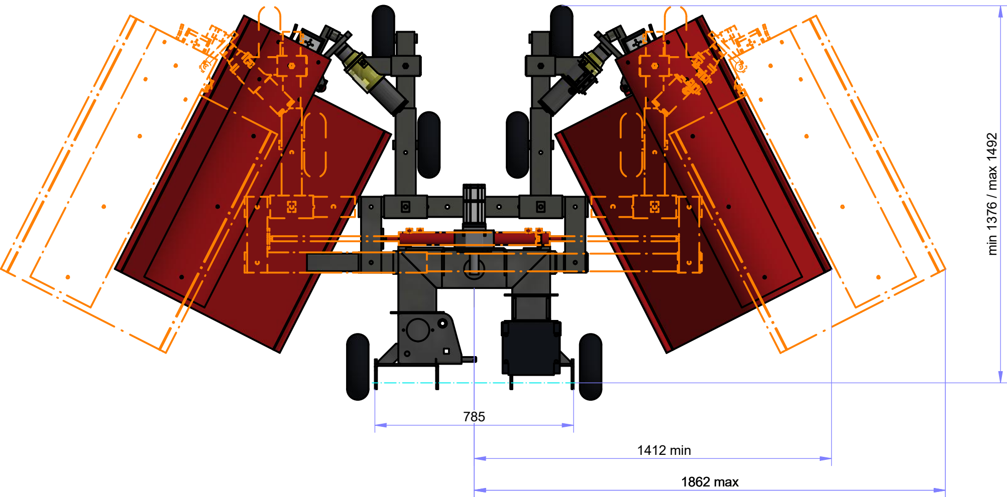
TOP VIEW ( 1 : 15 )
