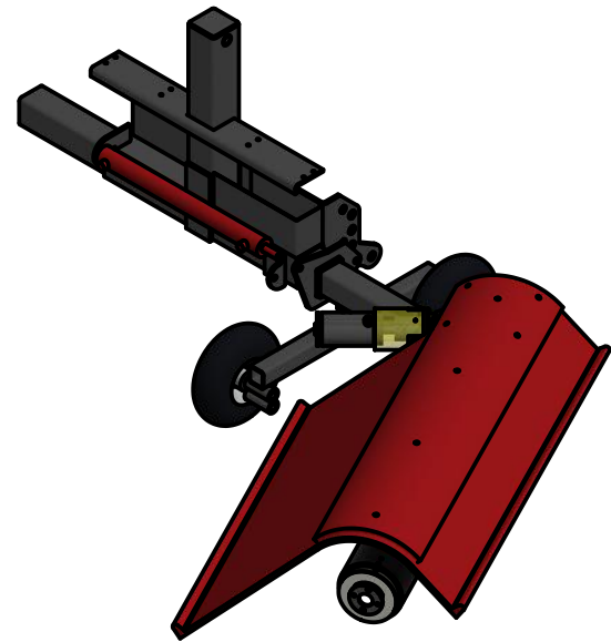
ISO VIEW ( 1 : 20 )
