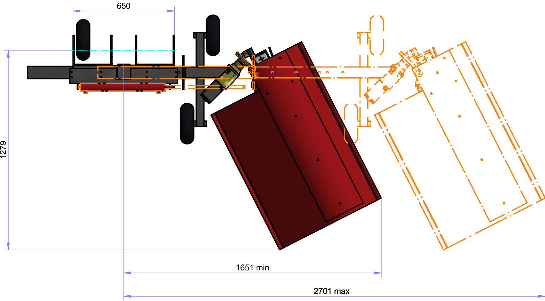
TOP VIEW ( 1 : 15 )
