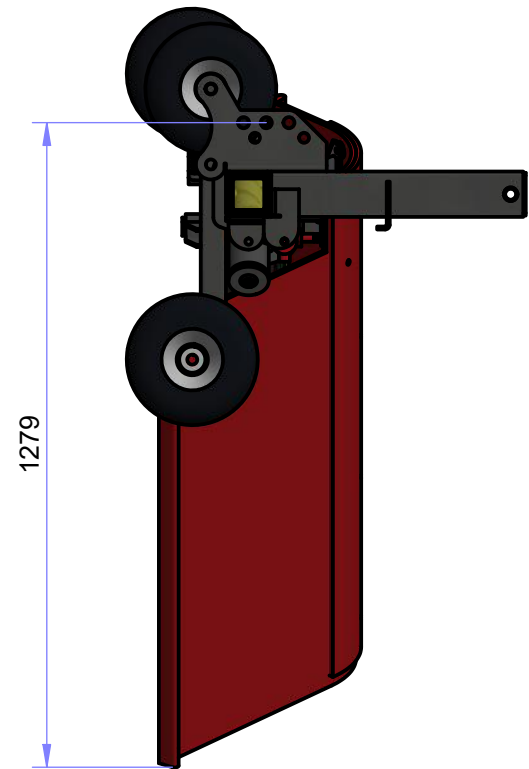
SIDE VIEW ( 1 : 15 )
