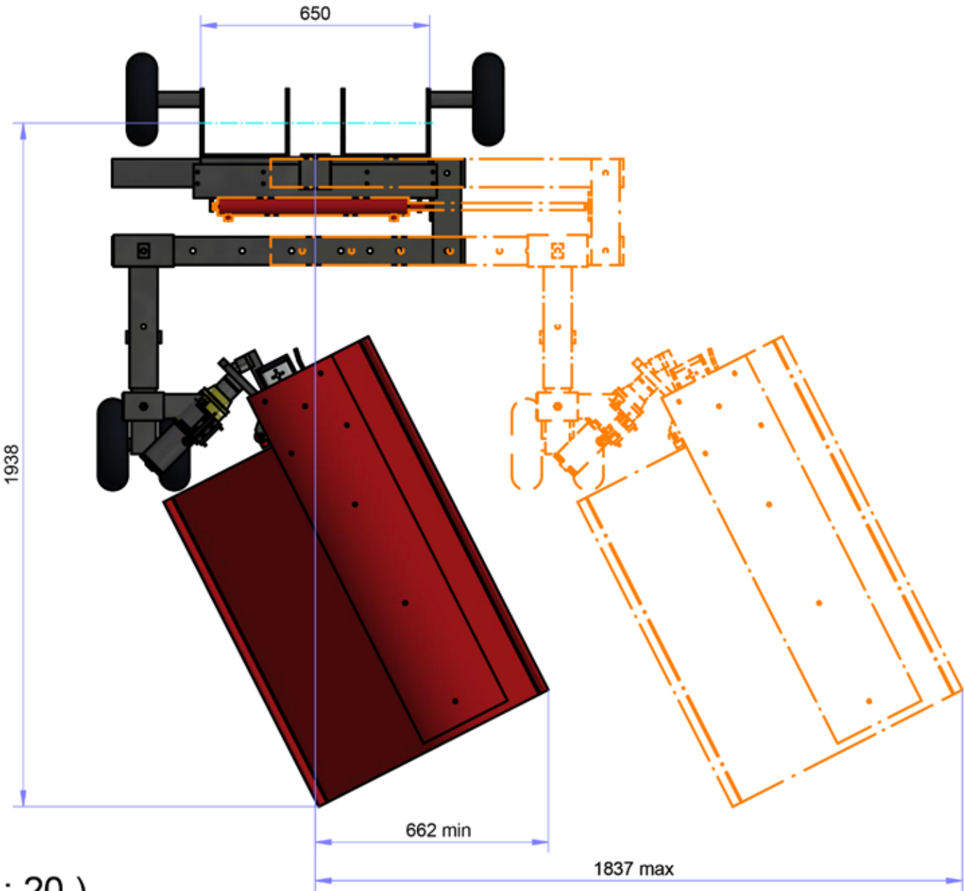
TOP VIEW ( 1 : 15 )
