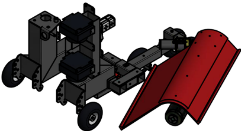
ISO VIEW ( 1 : 20 )
