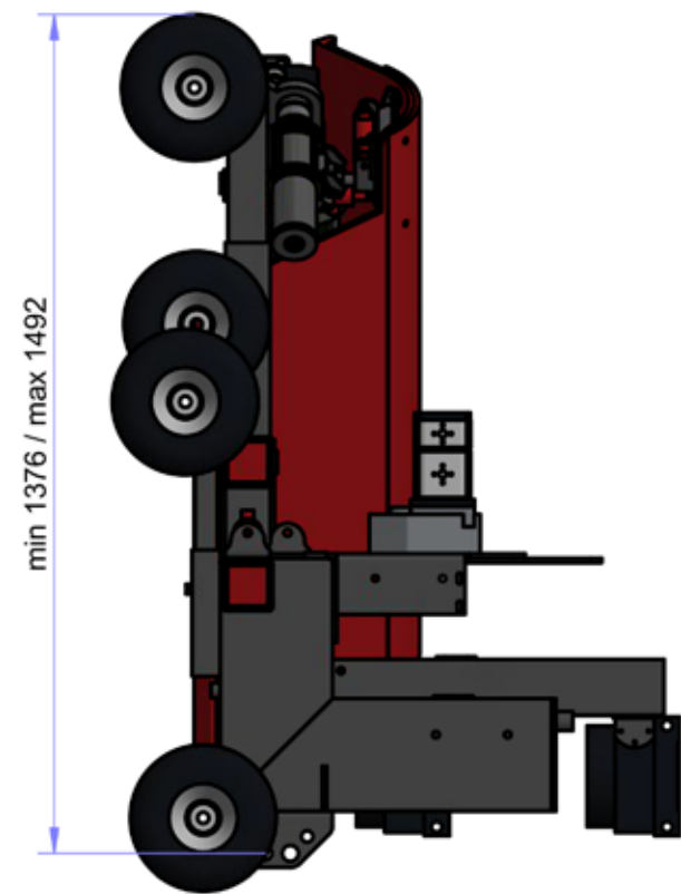
SIDE VIEW ( 1 : 15 )
