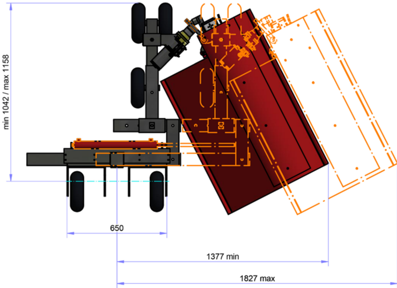
TOP VIEW ( 1 : 15 )
