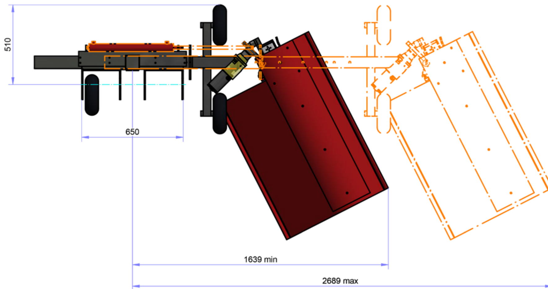
TOP VIEW ( 1 : 15 )
