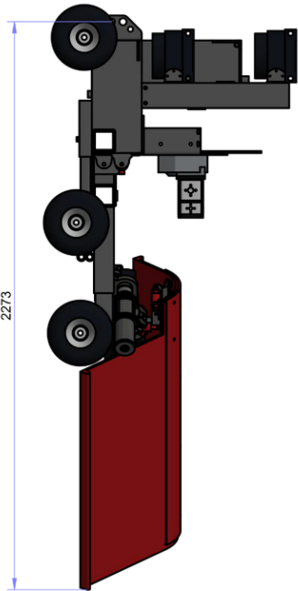
SIDE VIEW ( 1 : 15 )
