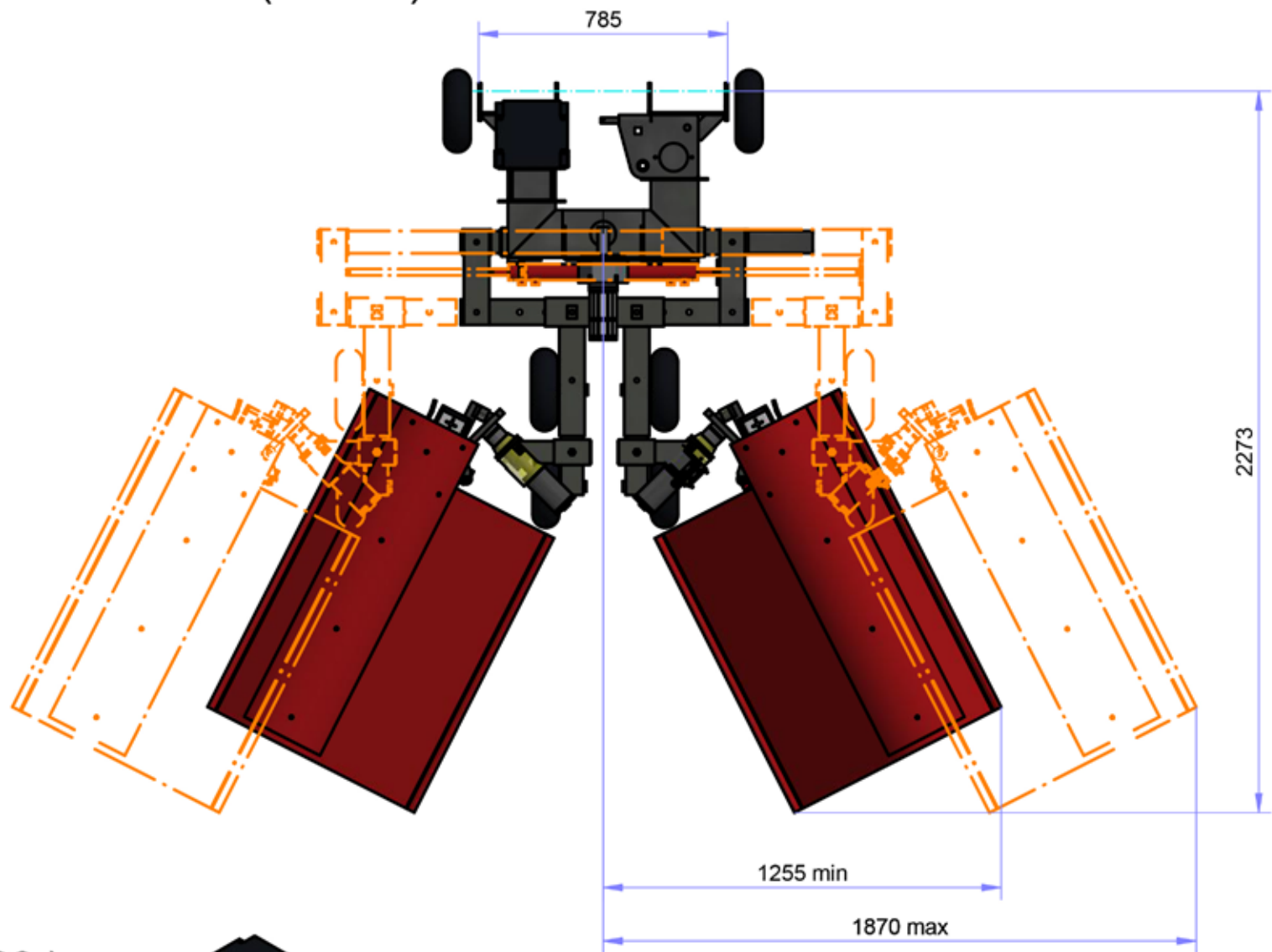
TOP VIEW ( 1 : 20 )
