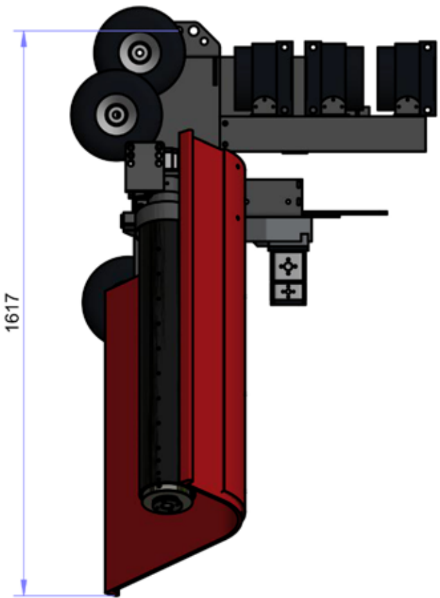
SIDE VIEW ( 1 : 15 )
