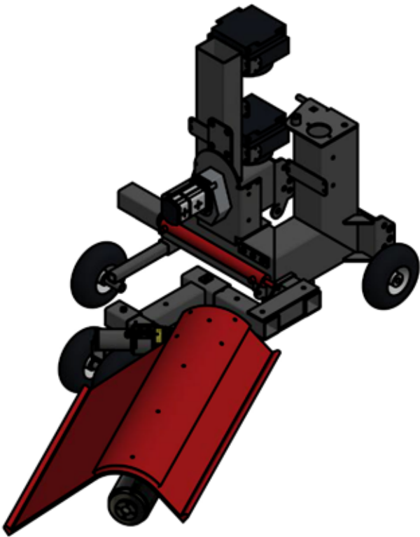
ISO VIEW ( 1 : 20 )
