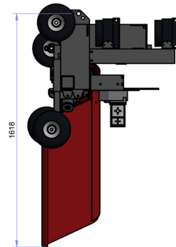
SIDE VIEW ( 1 : 15 )
