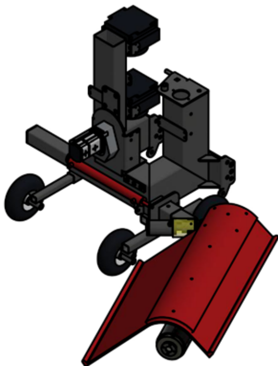
ISO VIEW ( 1 : 20 )
