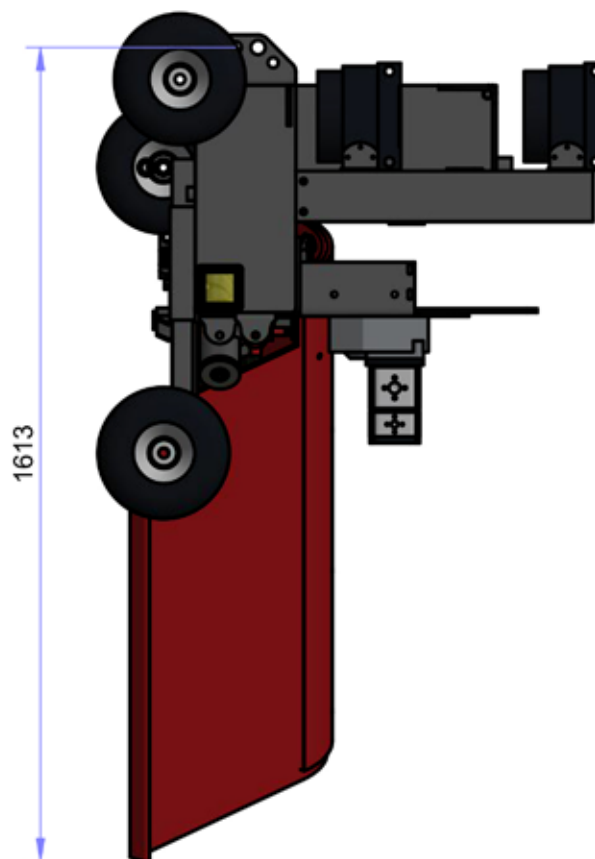
SIDE VIEW ( 1 : 15 )
