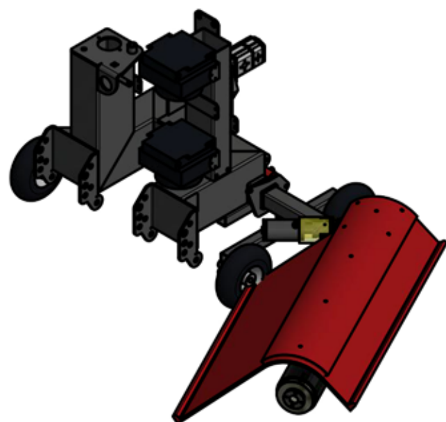
ISO VIEW ( 1 : 20 )
