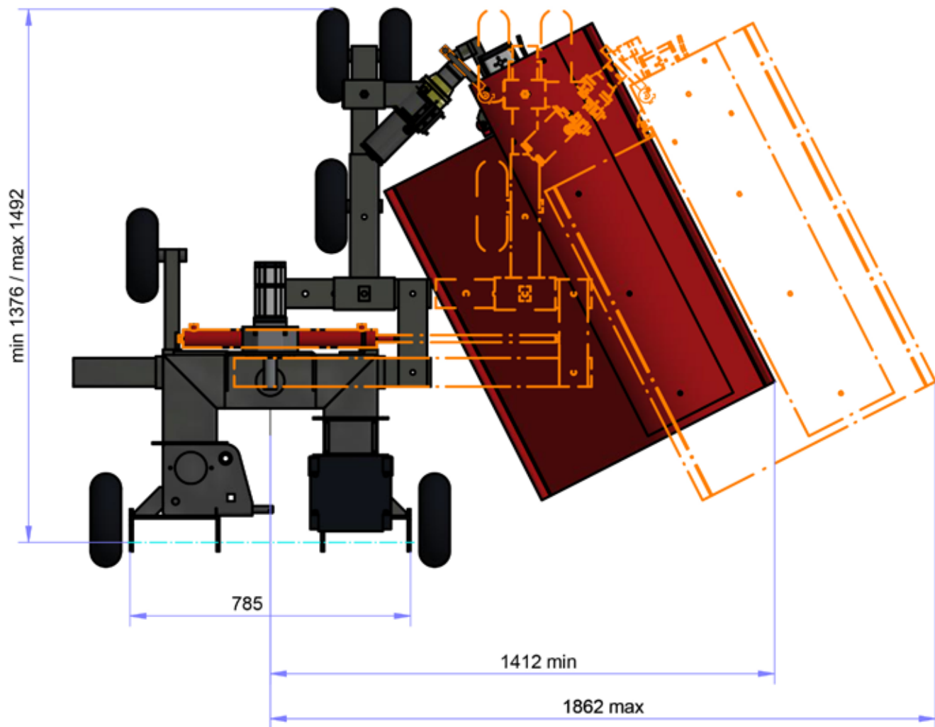
TOP VIEW ( 1 : 15 )
