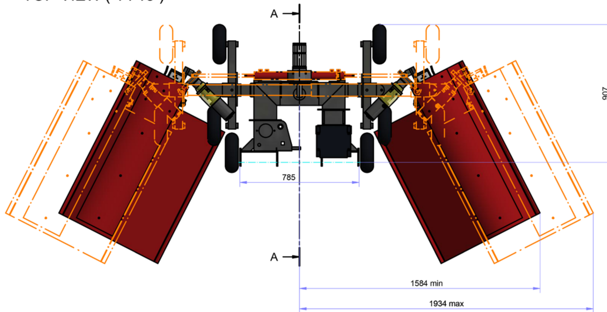
TOP VIEW ( 1 : 15 )
