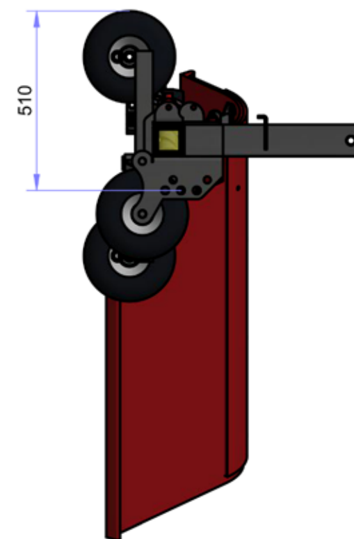
SIDE VIEW ( 1 : 15 )
