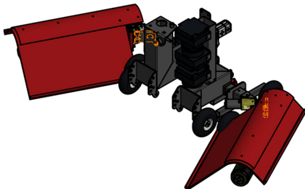
ISO VIEW ( 1 : 20 )
