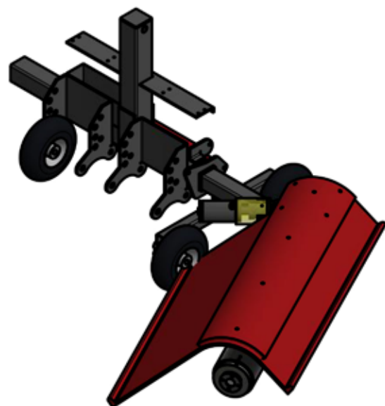
ISO VIEW ( 1 : 20 )
