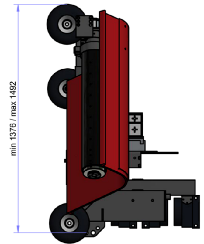
SIDE VIEW ( 1 : 15 )
