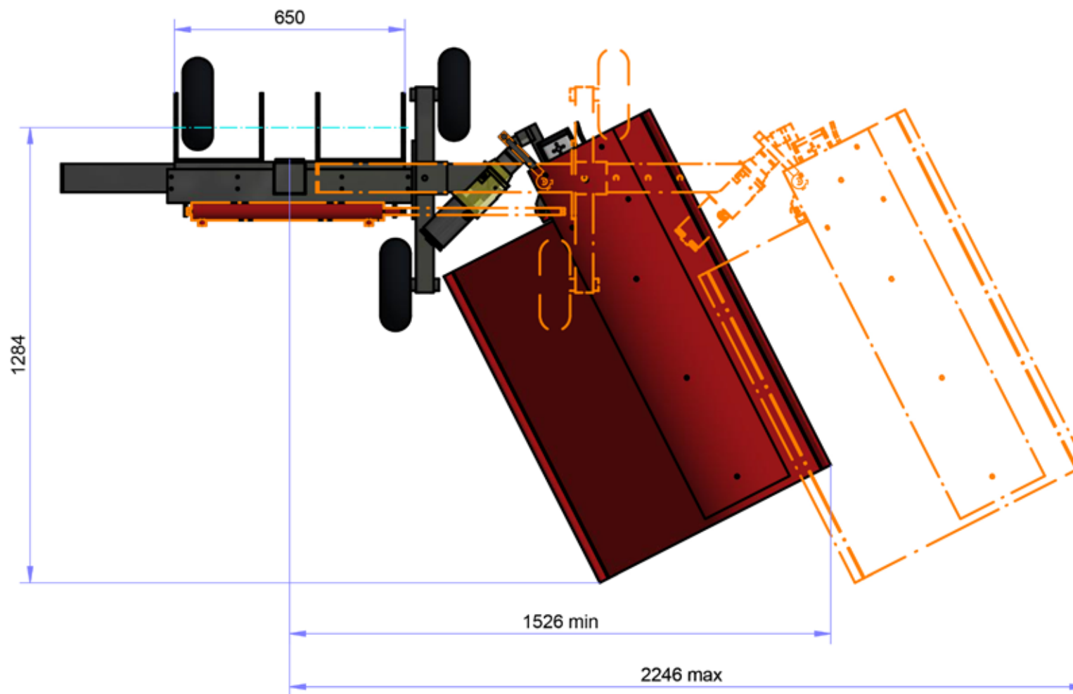
TOP VIEW ( 1 : 15 )
