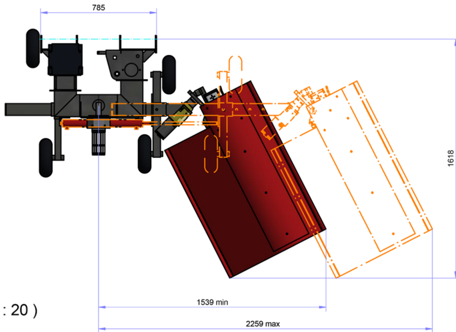
TOP VIEW ( 1 : 15 )
