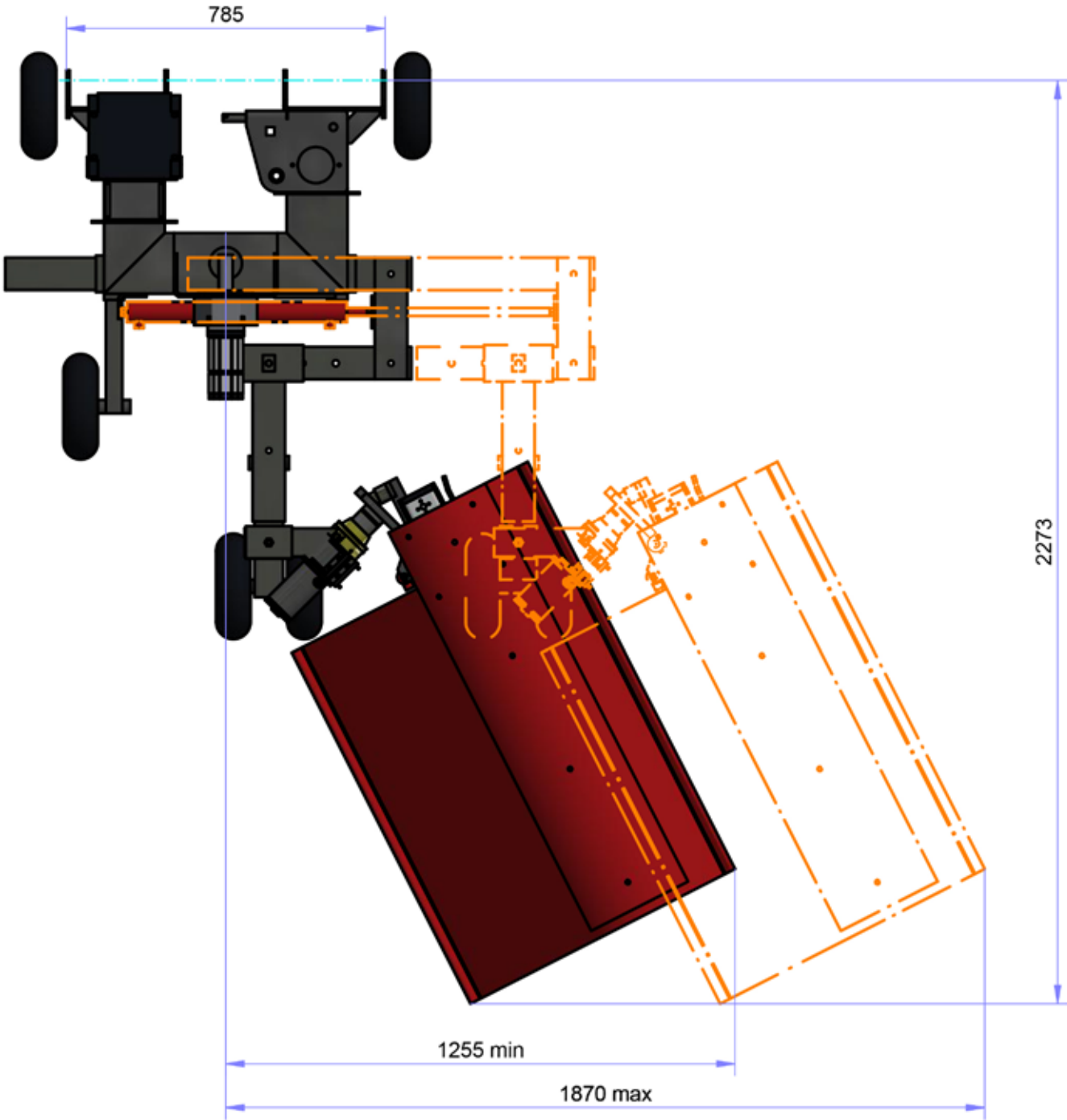
TOP VIEW ( 1 : 15 )
