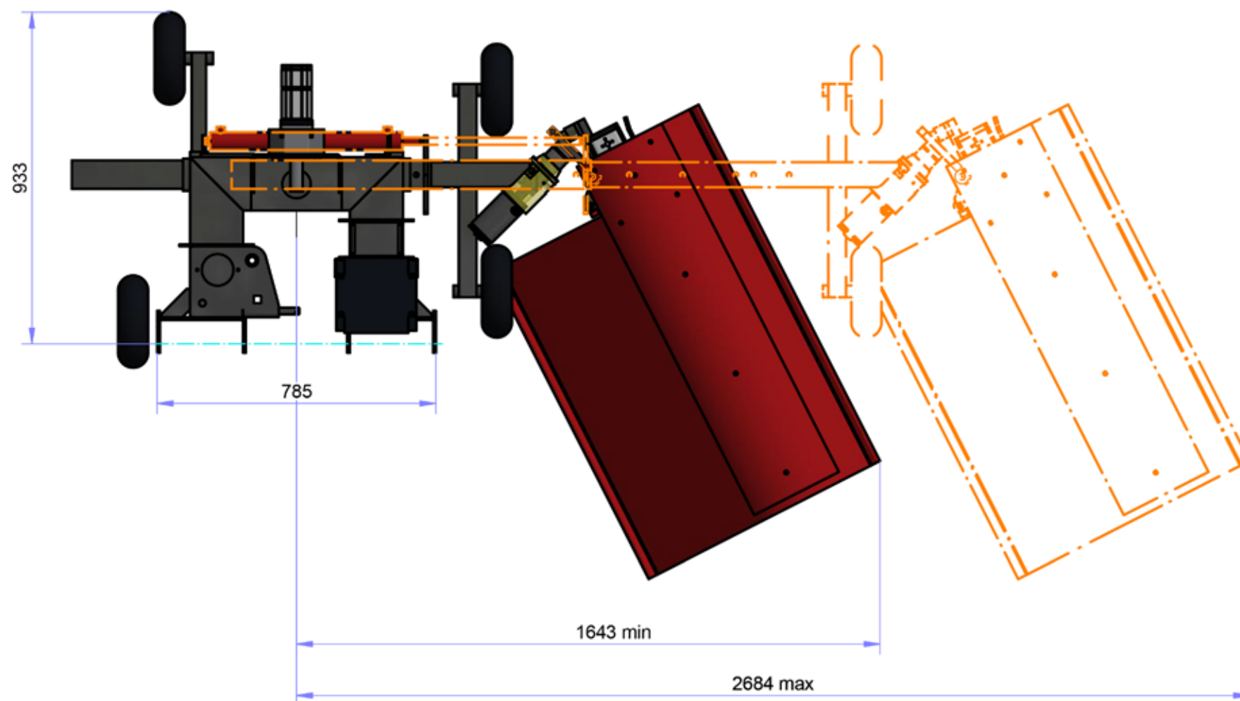
TOP VIEW ( 1 : 15 )
