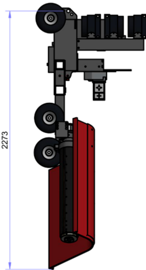
SIDE VIEW ( 1 : 20 )
