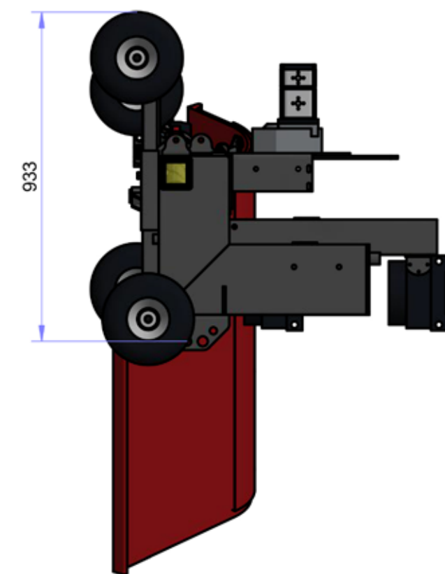
SIDE VIEW ( 1 : 15 )
