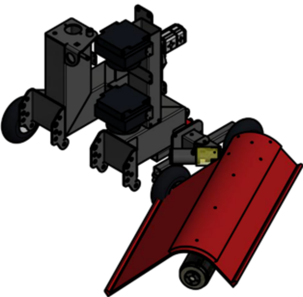
ISO VIEW ( 1 : 20 )
