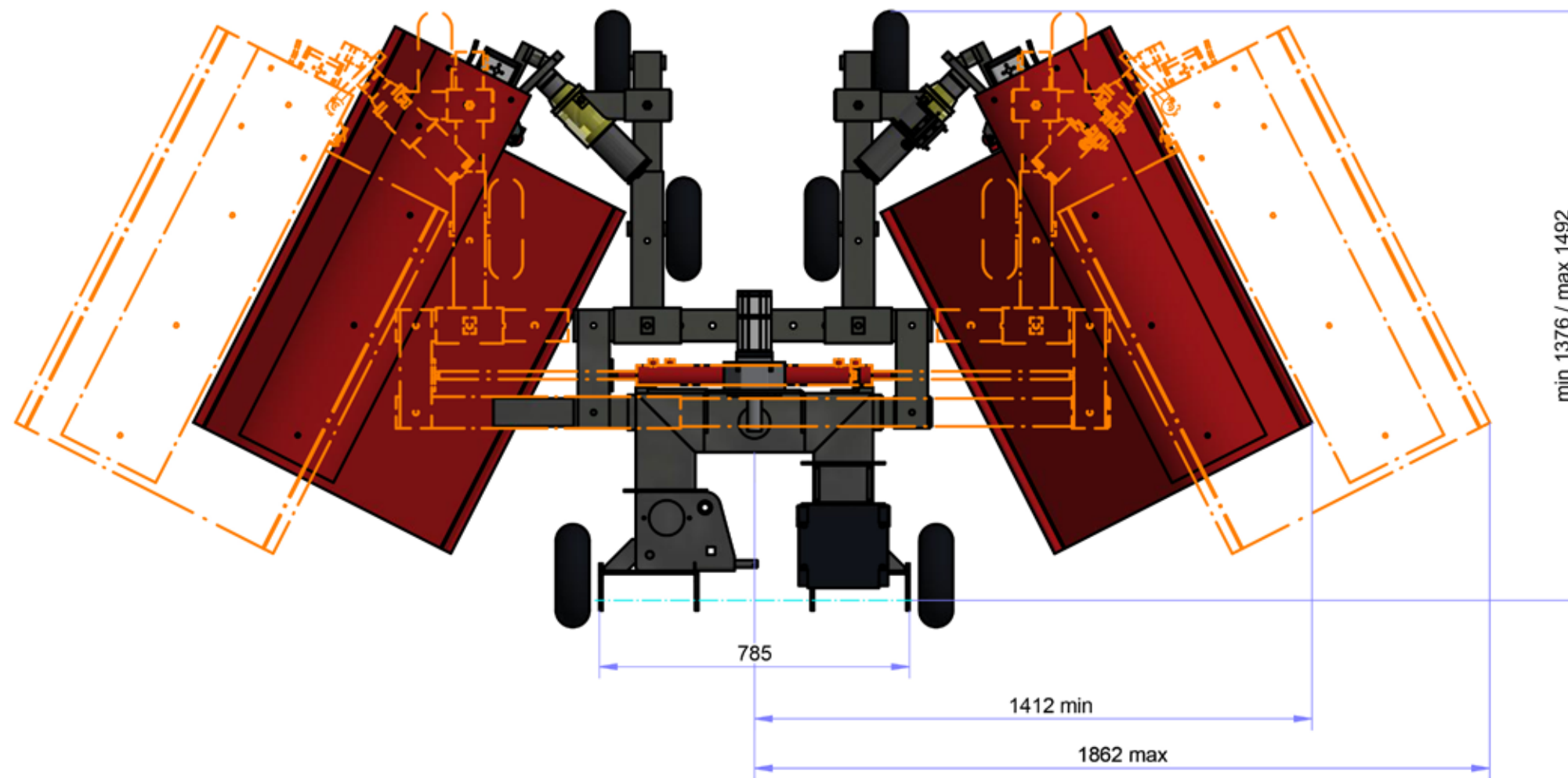
TOP VIEW ( 1 : 15 )
